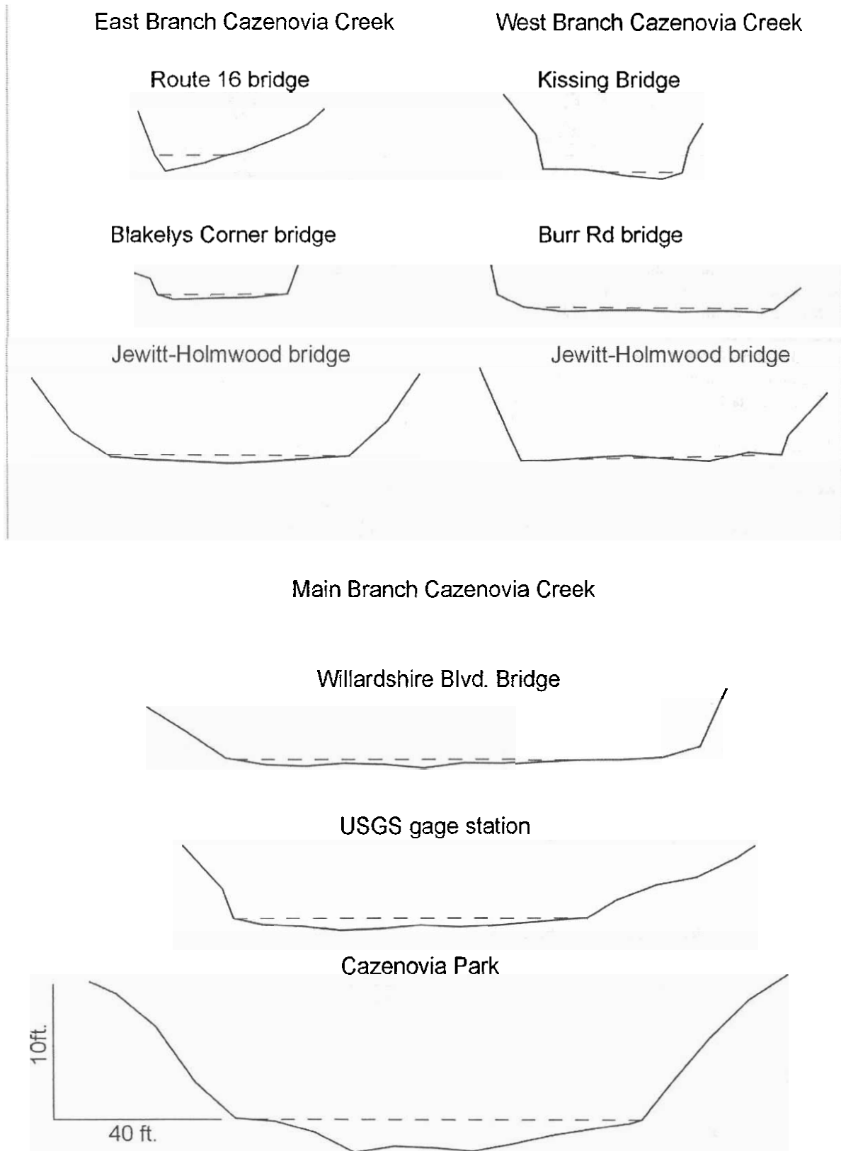
Figure 3. Cazenovia Creek cross section profiles. Dashed line is the water surface.
